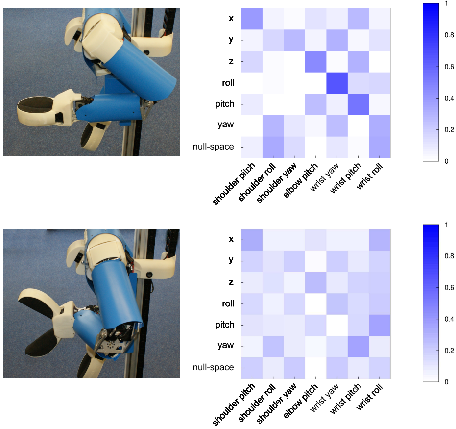
Fig. 3. Examples of activation matrices for two arm poses. The task-space dimensions correspond to forward/backward (x), lateral (y), vertical (z), and rotations around the x-axis (roll), y-axis (pitch), and z-axis (yaw).
